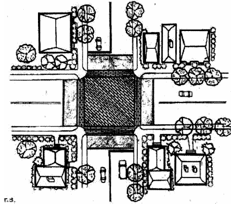
Raised intersection
